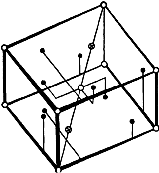
FIG. 3.—The structure of calcite. ⊗ represents Ca ++ ; ○ represents C; ● represents O.
